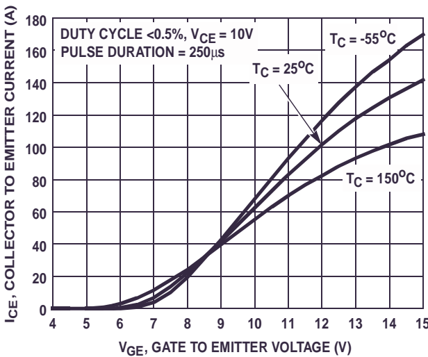
FIGURE 13. TRANSFER CHARACTERISTIC
