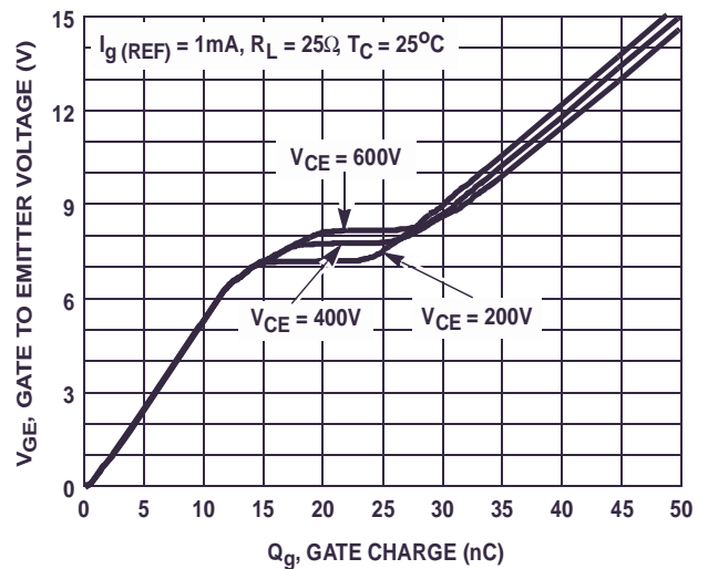
FIGURE 14. GATE CHARGE WAVEFORM
